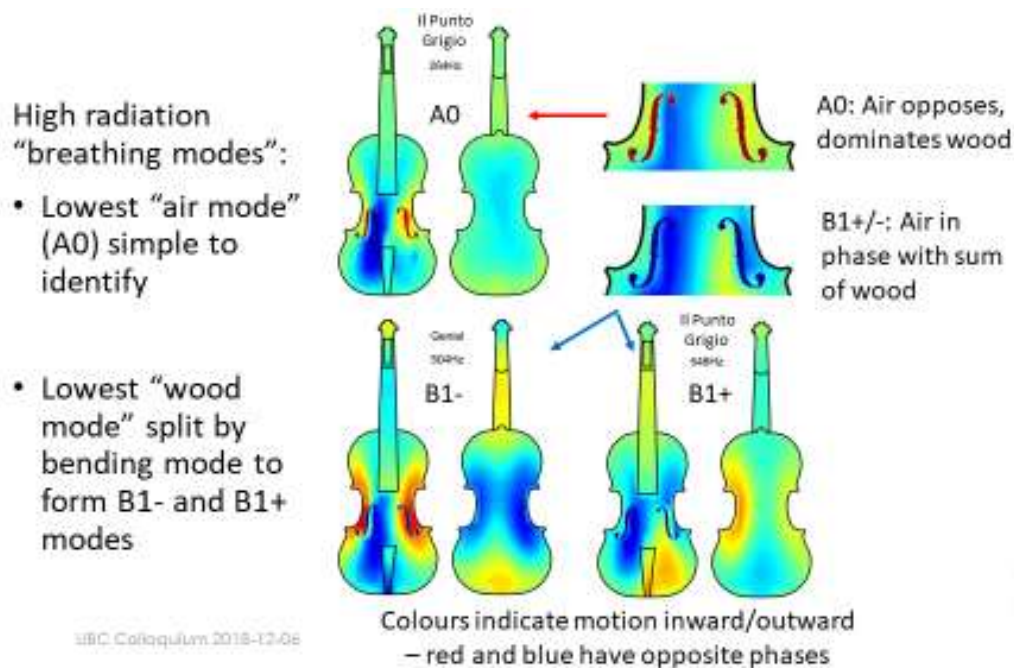
Figure 2: Shapes of signature vibration modes of a violin
