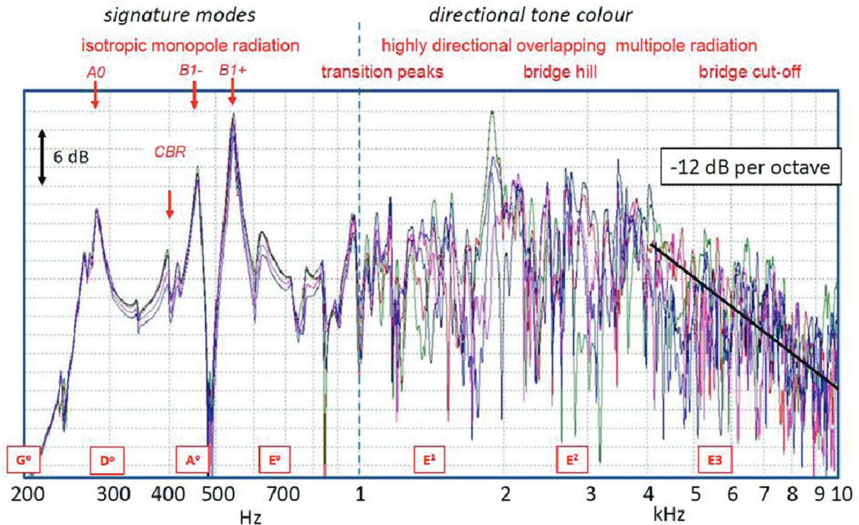
Figure 1: Radiated sound spectrum of the 1734 Willemotte Stradivari violin, from Colin Gough's article " Violin Acoustics " in Acoustic Today , summer 2016 (without permission).
